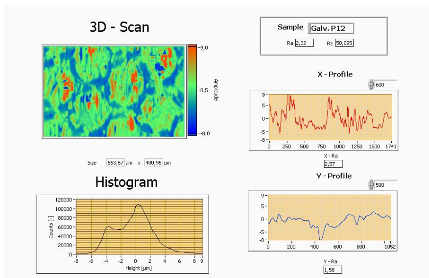
Fig. 3.2: On-line sensor moved in steps of 0.5 \mu\text{m} over a galvanized EBT surface to collect a 3d-data set. The unfiltered raw data are shown (dark-red and dark-blue are regions where no signal was detected). A microscopic image of the analyzed region is shown on the left.
